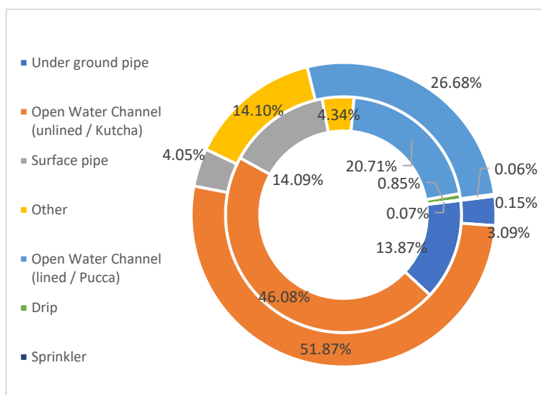
Chart 17: Percentage distribution of Ground Water (inner ring) and Surface Water (outer ring) Schemes by type of Water Distribution Methods
