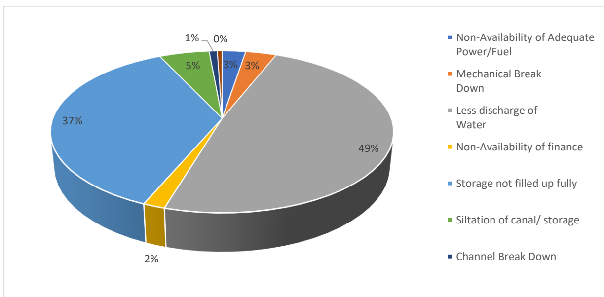
Chart 8: Reason- wise percentage share of ‘Temporarily Not-In Use’ Surface Water Schemes
