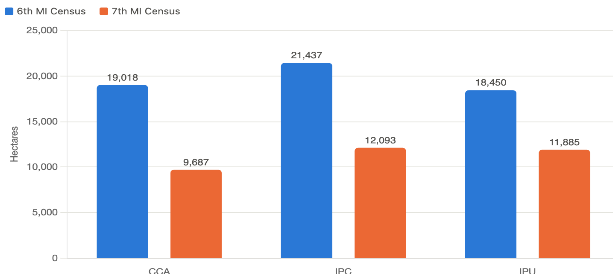
Chart 9: CCA, IPC and IPU for all MI Schemes — 7th vs 6th MI Census (in ha)
