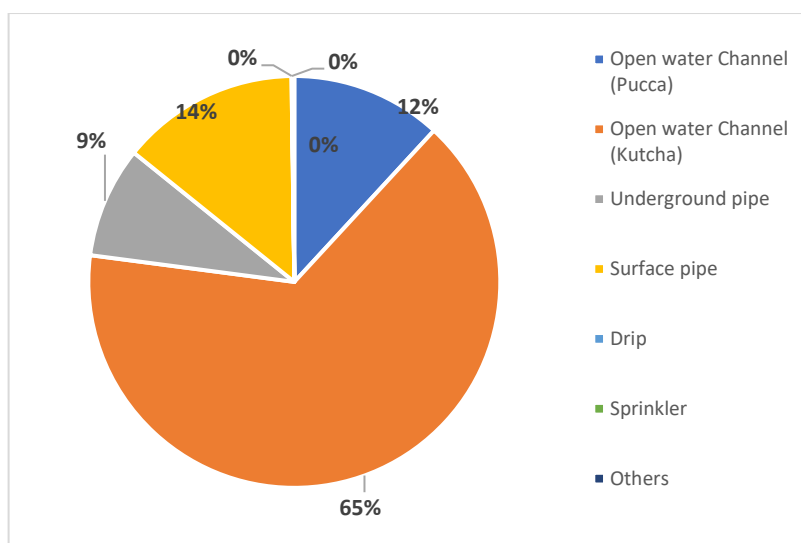
Chart 16: Percentage distribution of Ground Water (inner ring) and Surface Water (outer ring) Schemes by type of Water Distribution Methods
