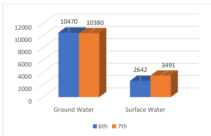
Chart 1: Number of Ground Water and Surface Water Schemes —7 th vs 6 th MI Census
