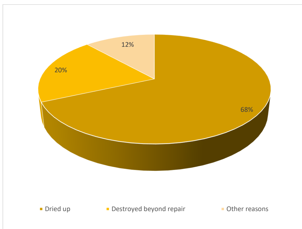
Chart 10: Reason-wise percentage distribution of ‘Permanently Not-In Use’ Ground-water Schemes
