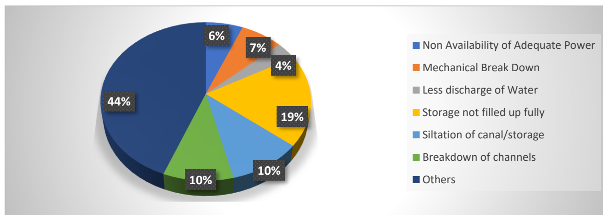
Chart 20: Percentage distribution of Surface Water schemes by reason for underutilisation
