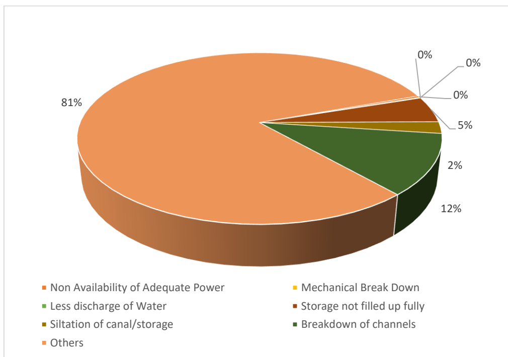
Chart 19: Percentage distribution of Surface Water schemes by reason for underutilisation
