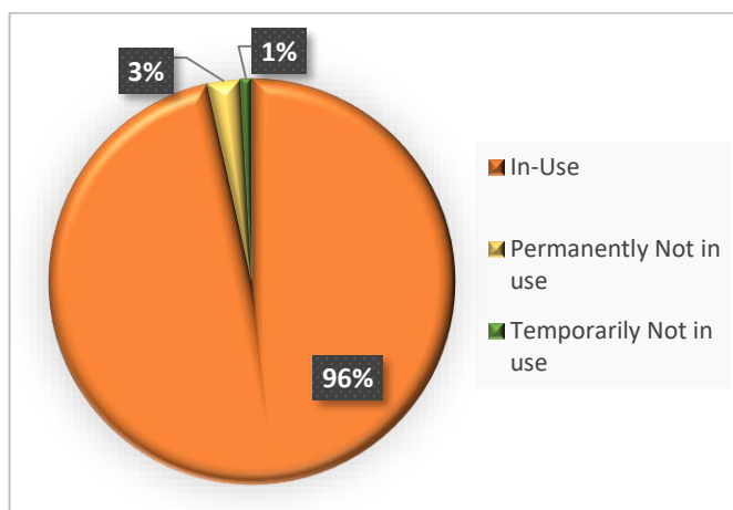
Chart 3: Percentage Share of 7 th MI Schemes by Usage Status
