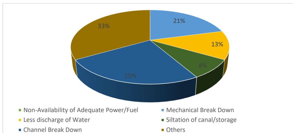
Chart 5: Reason- wise percentage share of ‘Temporarily Not-In Use’ Surface Water Schemes
