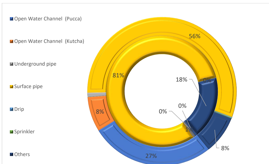
Chart 17: Percentage distribution of Ground Water (inner ring) and Surface Water (outer ring) Schemes by type of Water Distribution Methods
