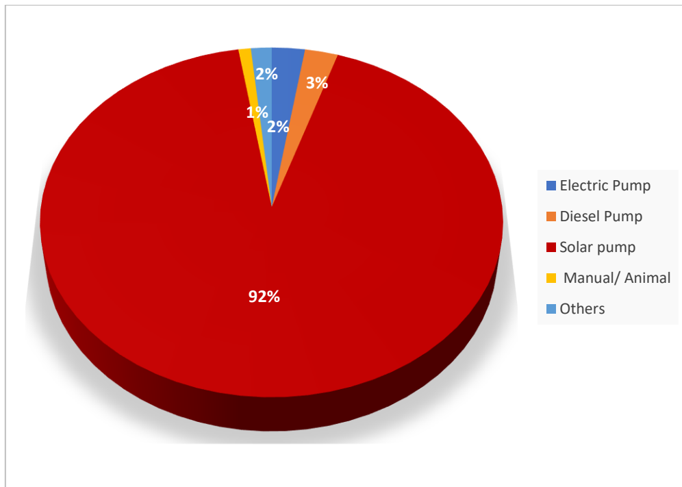
Chart 14: Percentage distribution of MI schemes by Source of Energy
