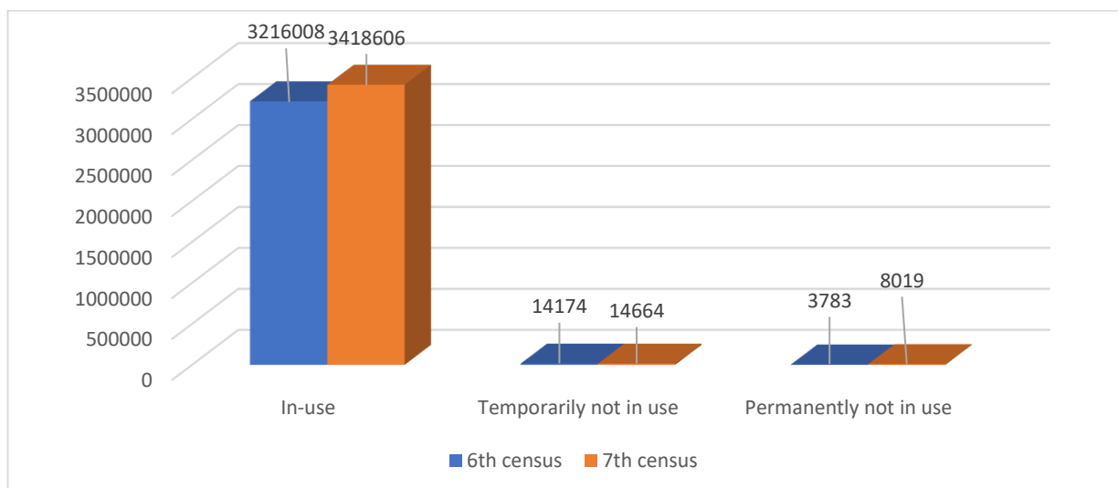
Chart 5: Number of Ground Water Schemes by Use status— 7th vs 6th MI Census
