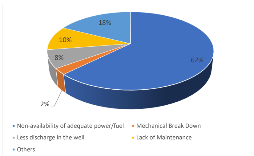
Chart 19: Percentage Distribution of Ground Water Schemes by Reason for Underutilisation
