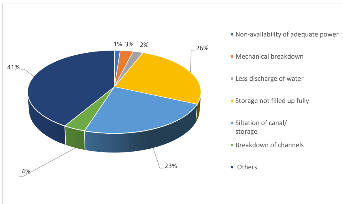
Chart 19: Percentage distribution of Surface Water schemes by reason for underutilisation
