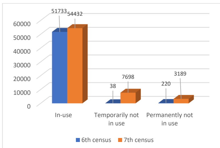
Chart 6: Number of Surface Water Schemes by Use status — 7th vs 6th MI Census
