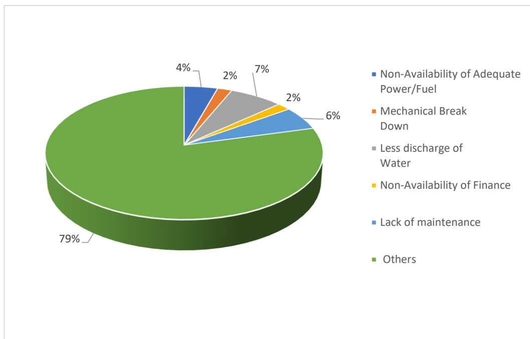
Chart 18: Percentage distribution of Ground Water schemes by reason for underutilisation
