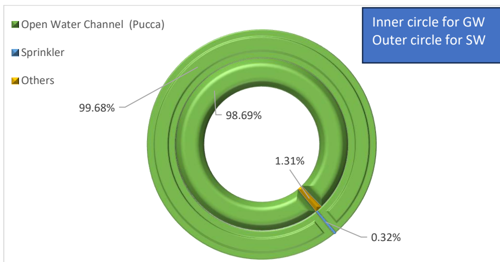
Chart 8: percentage distribution of Ground Water (inner ring) and Surface Water (outer ring) Schemes by type of Water Distribution Methods
