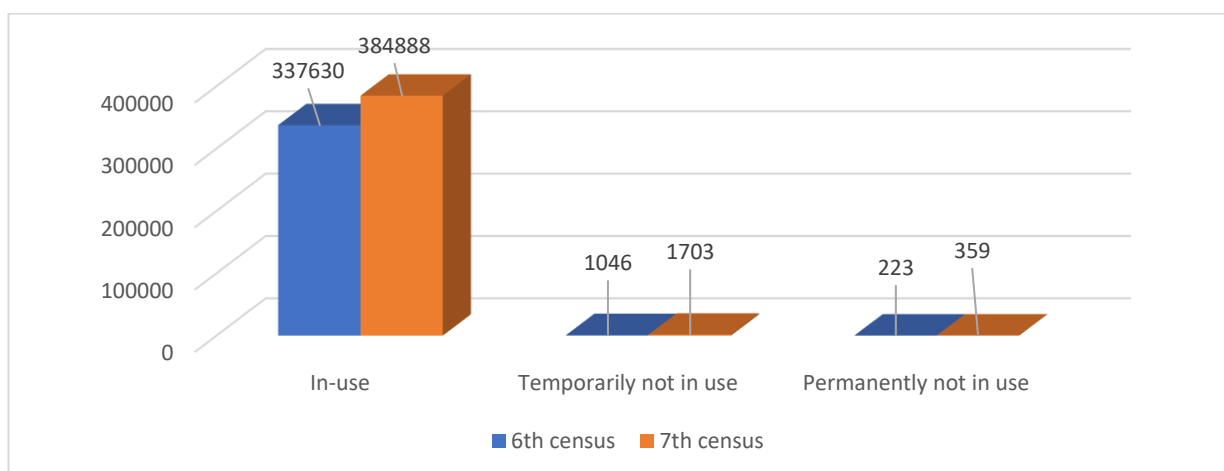
Chart 6: Number of Surface Water Schemes by Use status — 7th vs 6th MI Census
