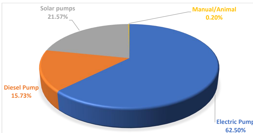
Chart 7: Percentage distribution of MI schemes by Source of Energy
