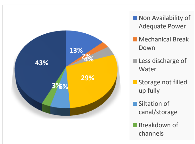
Chart 18: Percentage distribution of Surface Water schemes by reason for underutilisation
