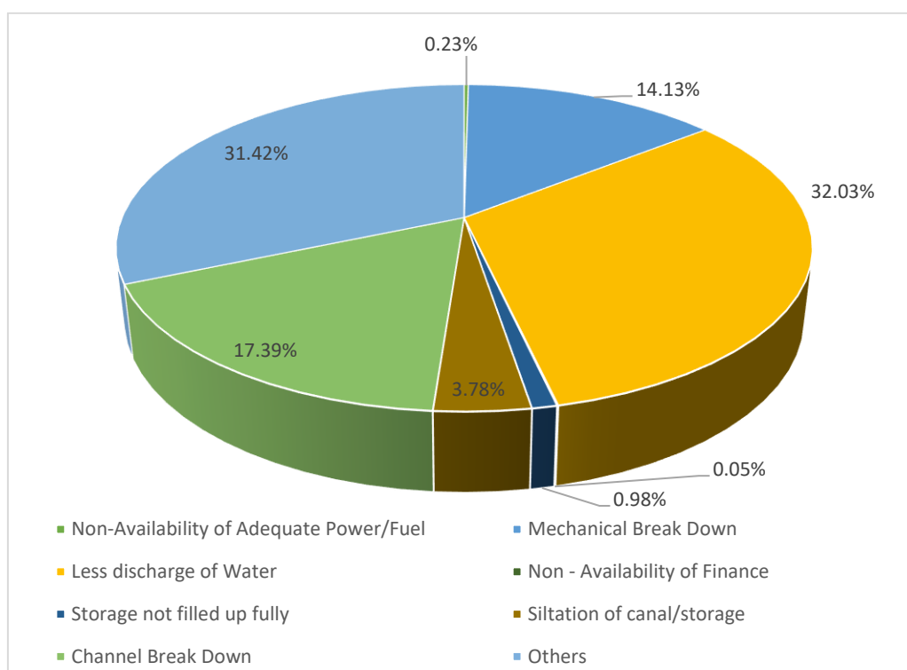
Chart 9: Reason- wise percentage share of ‘Temporarily Not-In Use’ Surface Water Schemes
