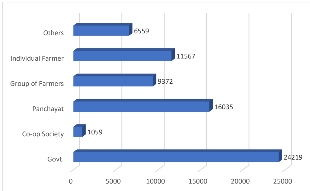
Chart 13: Ownership of Surface Water Schemes (Number)
