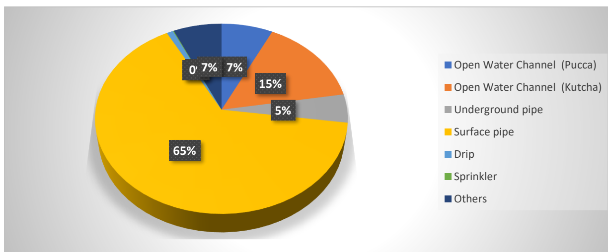
Chart 16: percentage distribution of Ground Water
