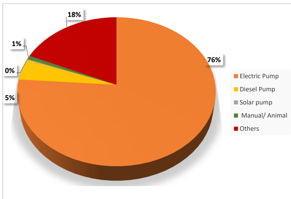
Chart 14: Percentage distribution of MI schemes by Source of Energy
