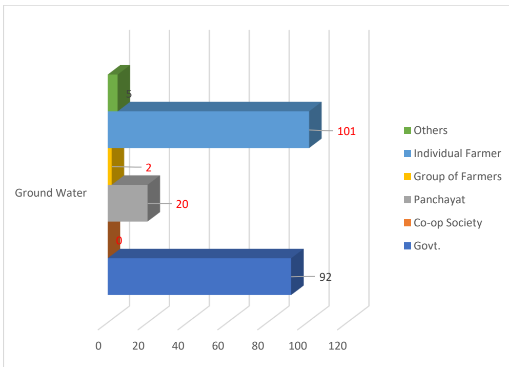
Chart 13: Ownership of Ground Water Schemes (Number)
