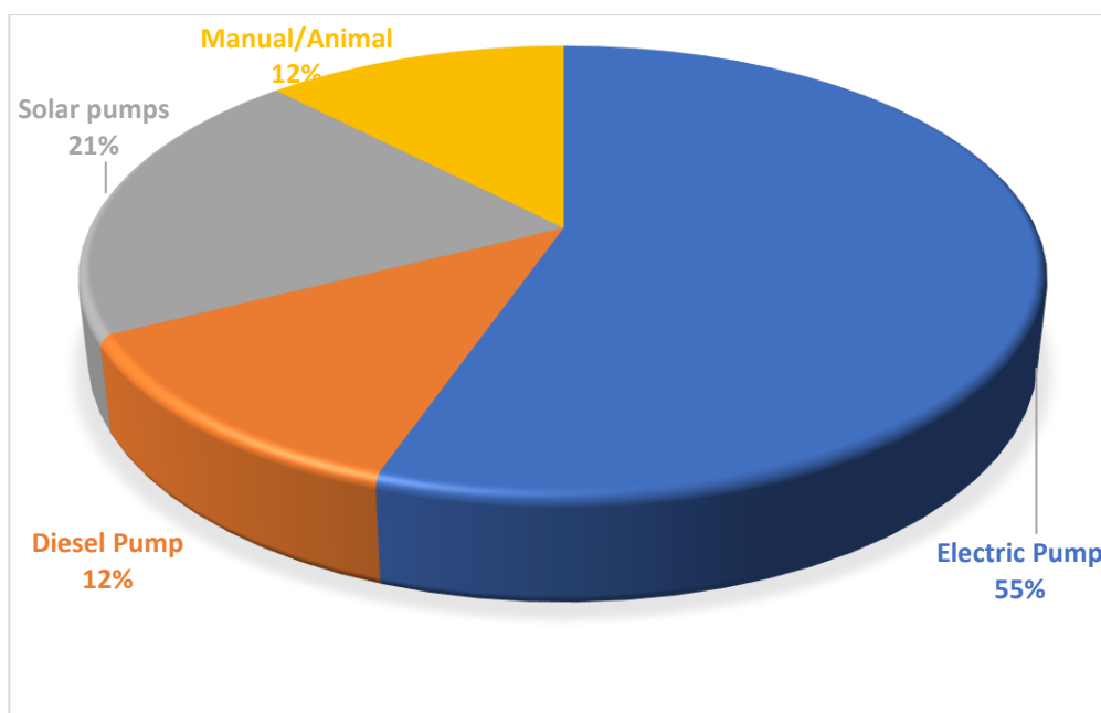
Chart 15: Percentage distribution of MI schemes by Source of Energy
