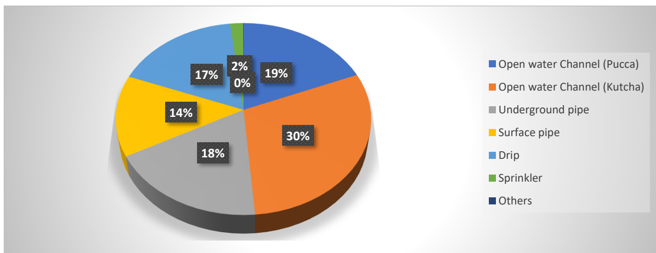
Chart 16: Percentage distribution of MI Schemes by type of Water Distribution Methods
