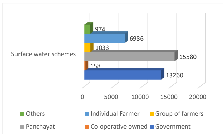
Chart 13: Ownership of Surface Water Schemes (Number)
