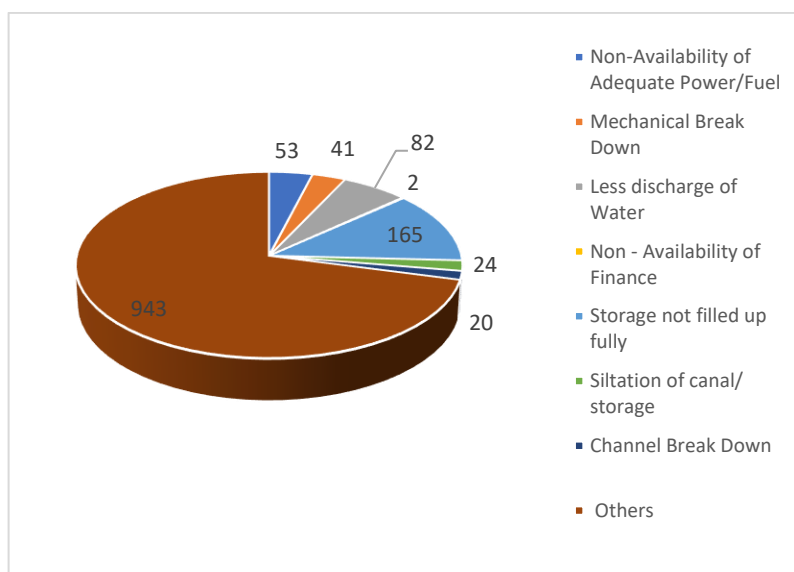
Chart 8: Number of ‘Temporarily Not in Use’ Surface Water Schemes
