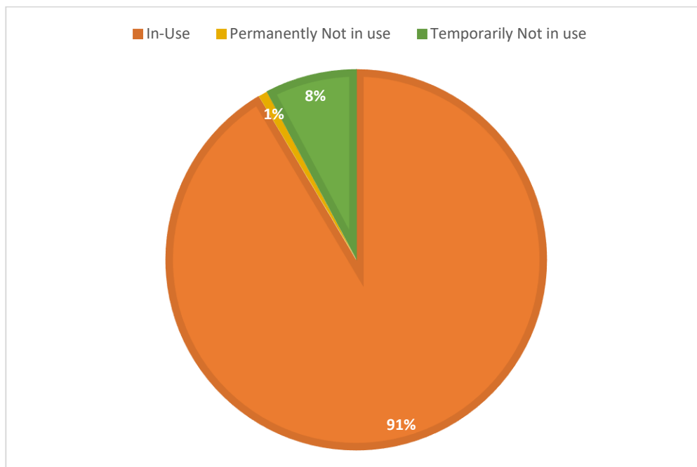
Chart 3: Percentage Share of 7 th MI Schemes by Usage Status
