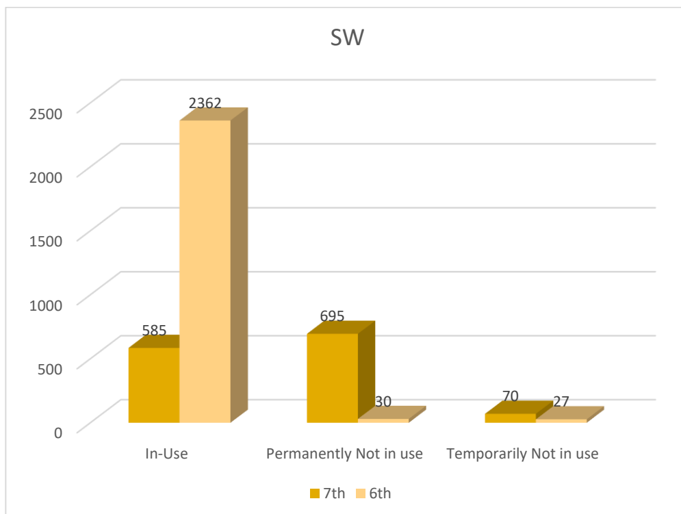
Chart 5: Number of Ground Water Schemes by Use status— 7 th vs 6 th MI Census
