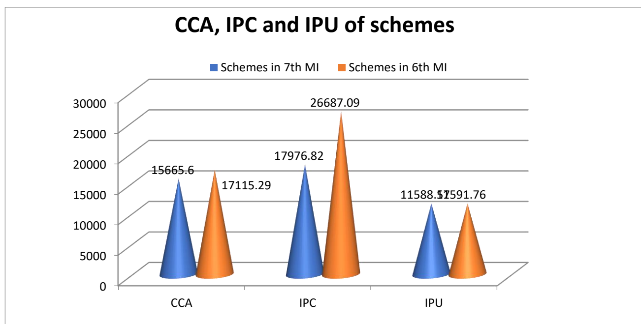
Chart 18: CCA, IPC and IPU for all MI Schemes — 7th vs 6th MI Census
