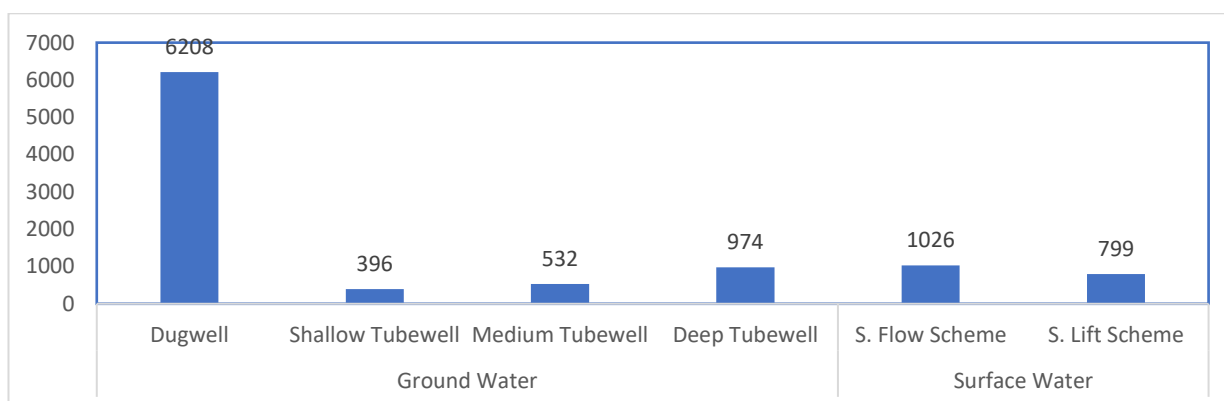
Chart 21: Number of Schemes used for Ground Water Recharge
