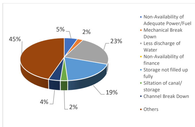
Chart 8: Reason- wise percentage share of ‘Temporarily Not-In Use’ Surface Water Schemes
