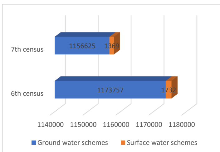
Chart 1: Number of Ground Water and Surface Water Schemes —7 th vs 6 th MI Census
