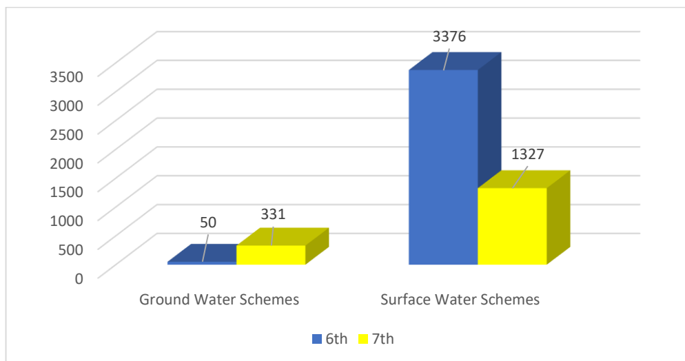
Chart 1: Number of Ground Water and Surface Water Schemes 6 th vs 7 th MI Census
