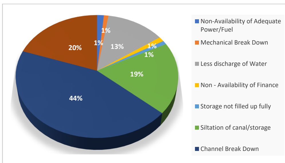
Chart 8: Reason-wise percentage distribution of ‘Temporarily Not-In Use’ Surface-water Schemes
