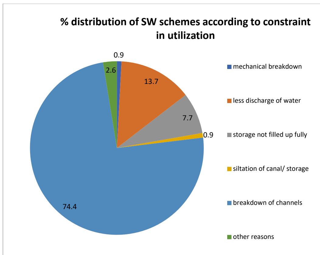
Chart 19: Percentage distribution of Surface Water schemes by reason for underutilisation
