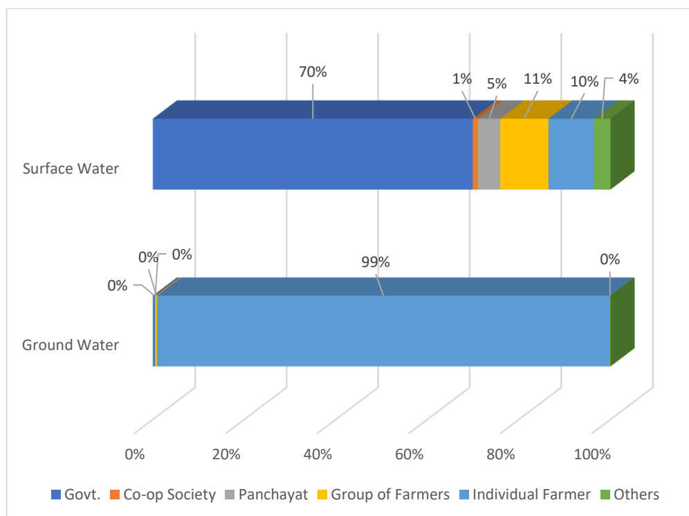
Chart 12: Ownership of Ground Water Schemes (Number)
