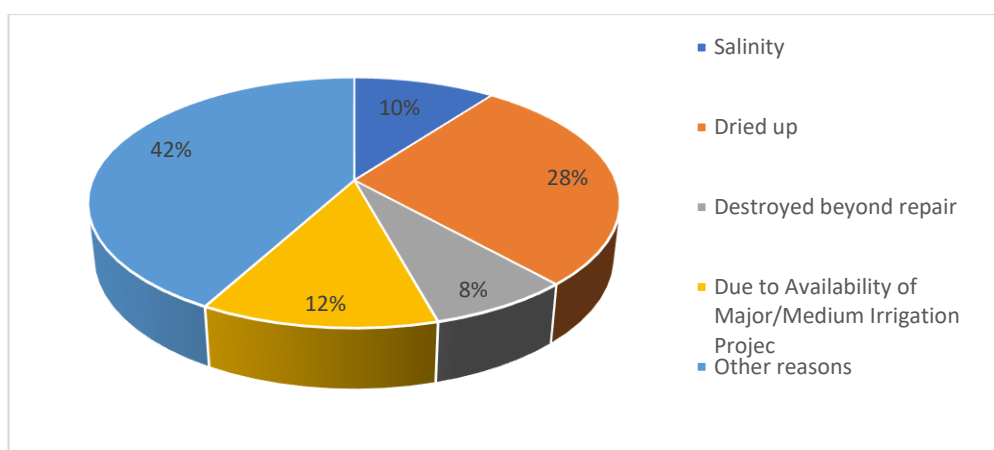
Chart 10: Reason wise percentage distribution of ‘Permanently Not-In Use’ Surface Water Schemes
