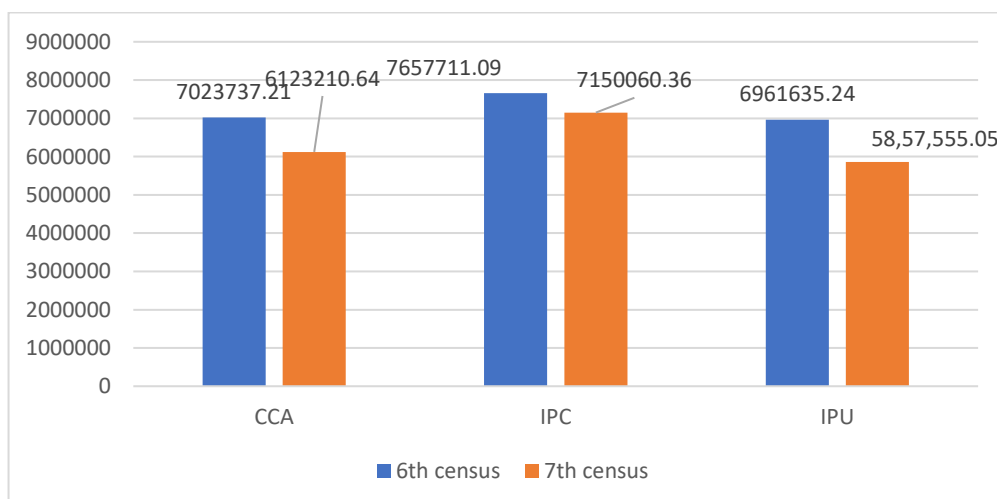
Chart 16: CCA, IPC and IPU for all MI Schemes — 7 th vs 6 th MI Census
