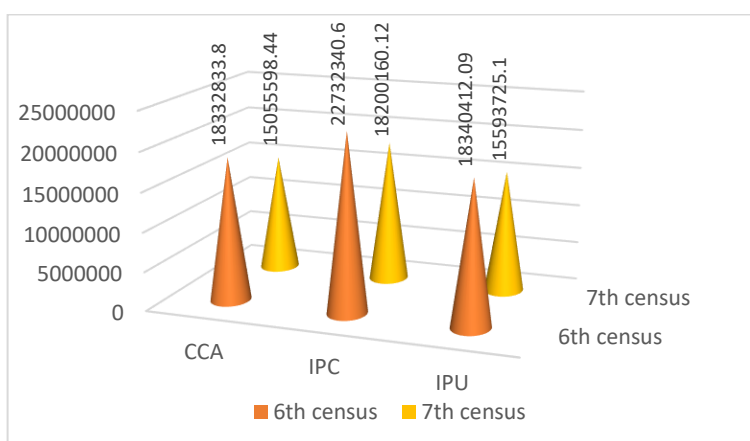
Chart 17: CCA, IPC and IPU for all MI Schemes — 7th vs 6th MI Census (in ha)
