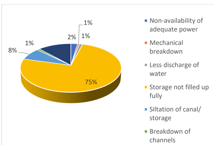
Chart 19: Percentage distribution of Surface Water schemes by reason for underutilisation
