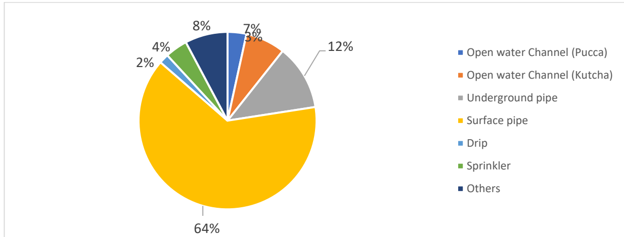
Chart 16: Percentage distribution of Schemes by type of Water Distribution Methods
