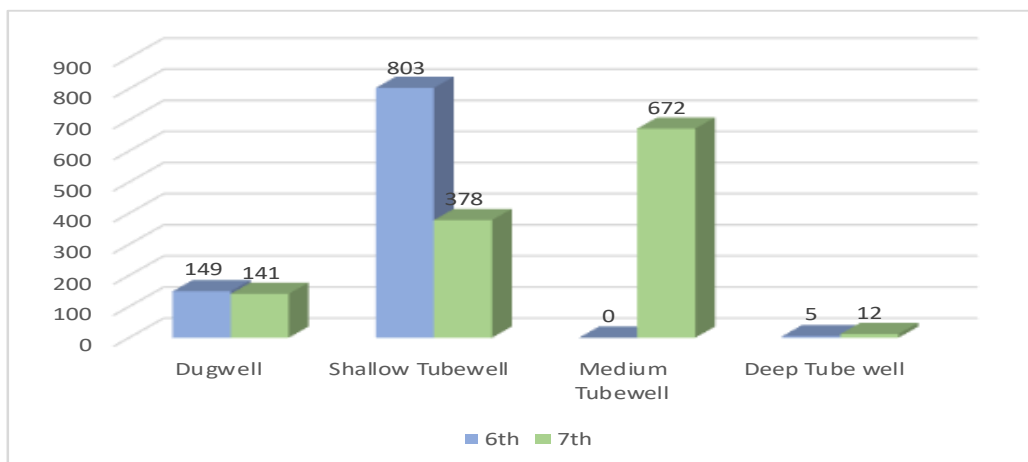
Chart 2: Number of Ground Water Schemes by Type —7 th vs 6 th MI Census
