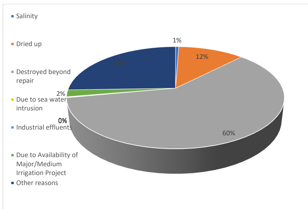
Chart 11: Reason wise percentage distribution of ‘Permanently Not-In Use’ Surface Water Schemes
