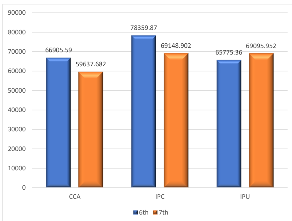
Chart 17: CCA, IPC and IPU for all MI Schemes — 7th vs 6th MI Census
