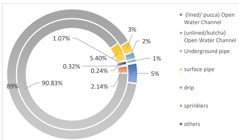
Chart 17: Percentage distribution of Ground Water (inner ring) and Surface Water (outer ring) Schemes by type of Water Distribution Methods
