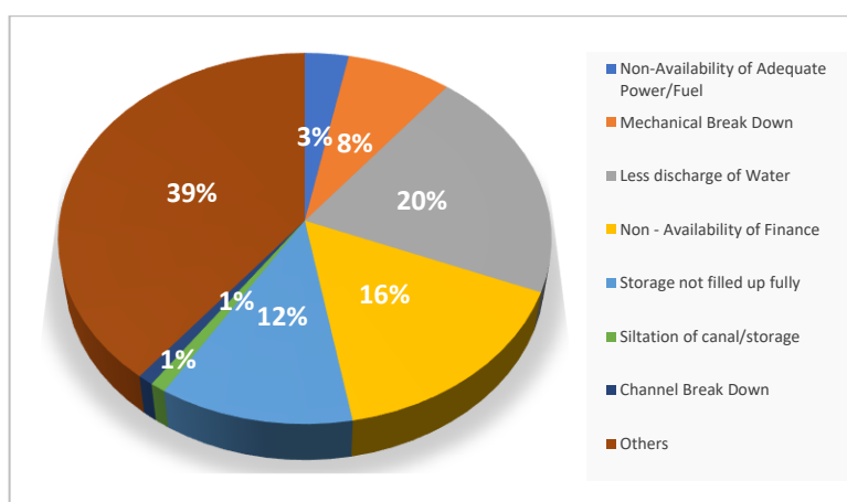
Chart 7: Reason-wise percentage distribution of ‘Temporarily Not-In Use’ Surface-water Schemes
