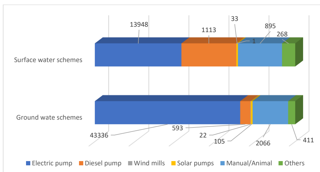
Chart 15: Number of Ground Water vs Surface Water Schemes by Source of Energy
